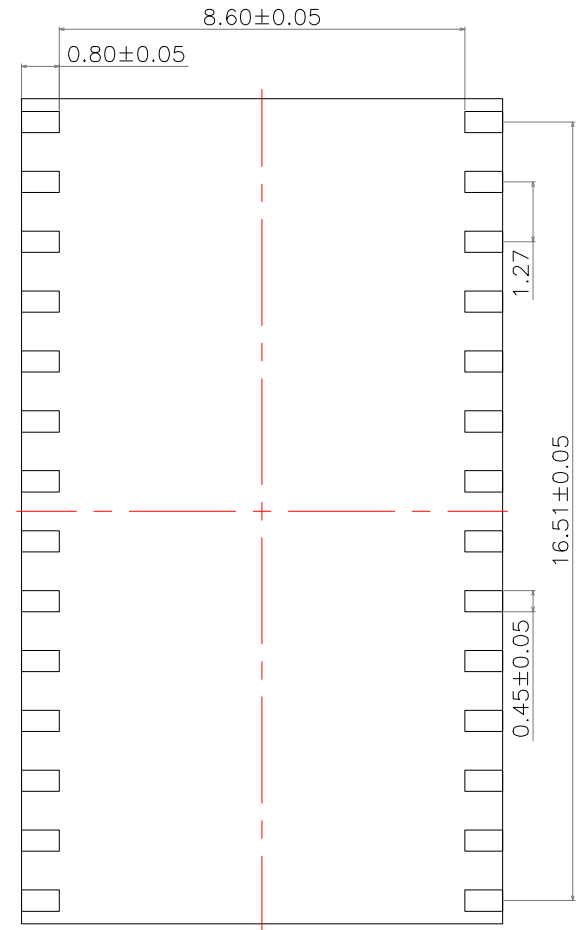
BOTTOM VIEW
